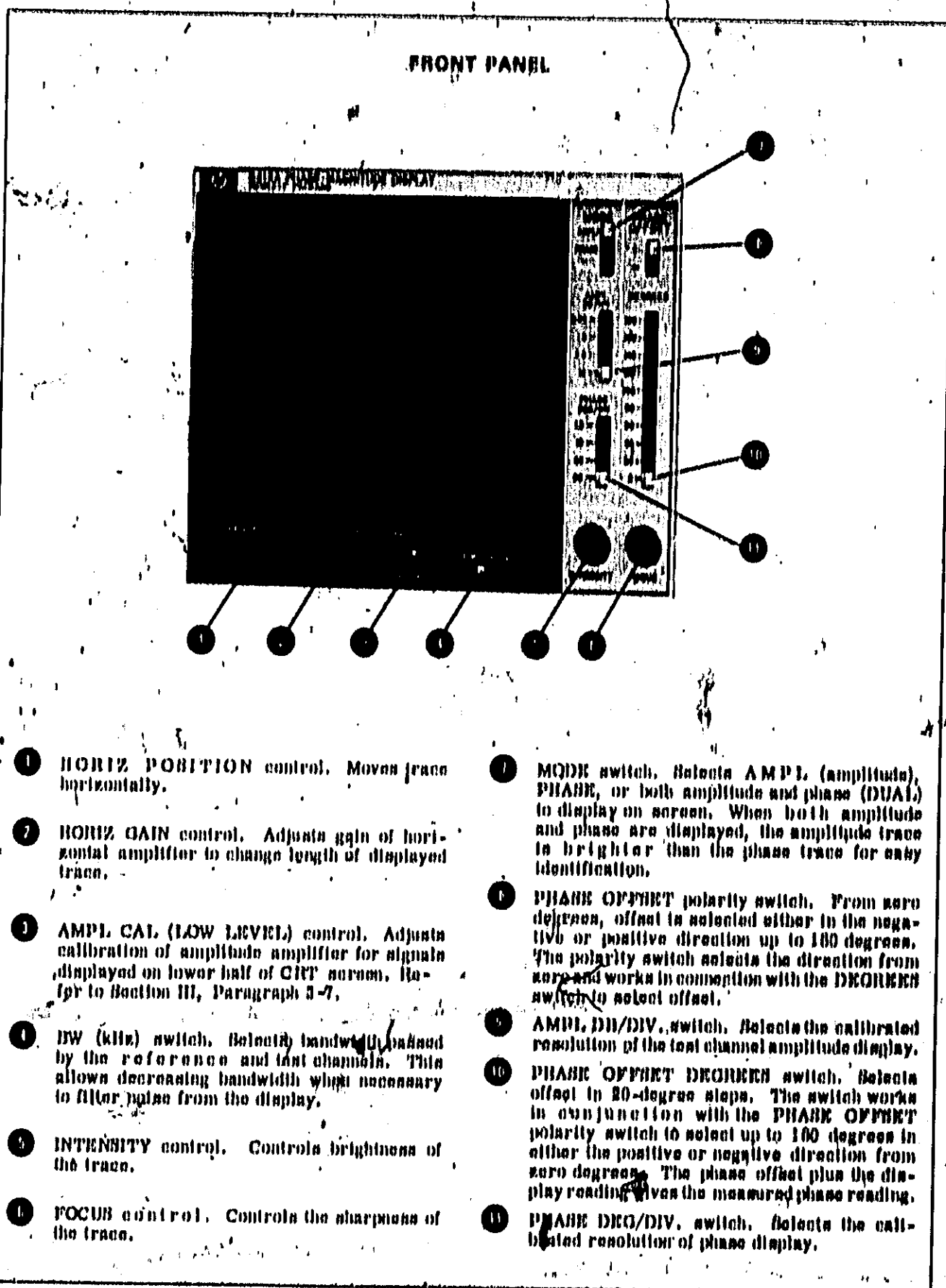
Figure 5-1. Model 0412A Front Panel Features
